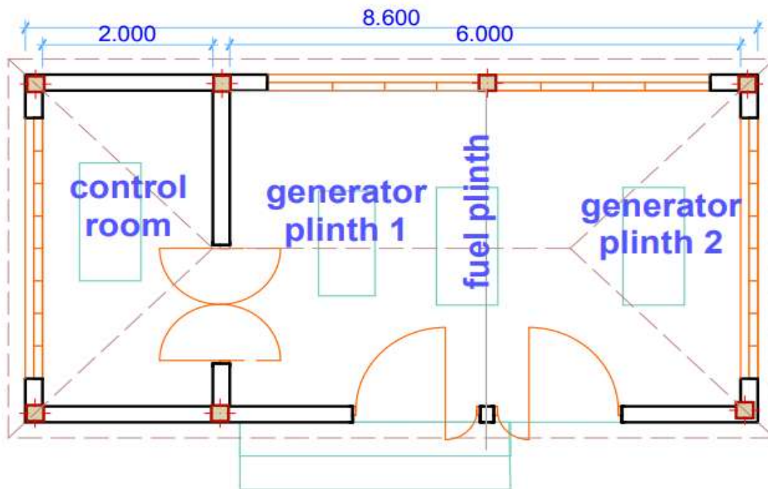
Plane of generator room
